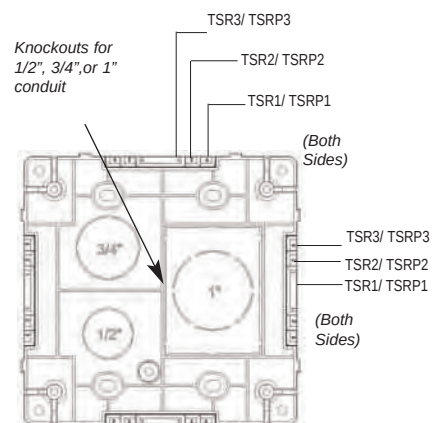
JBD, JBD2 - DUAL GANG
